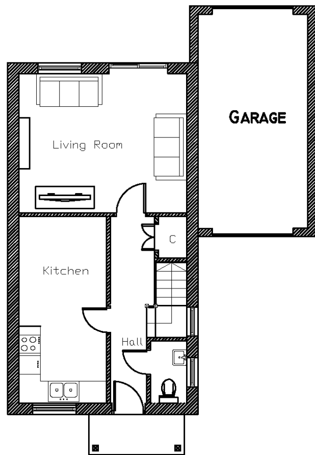
PROPOSED GROUND FLOOR PLAN @ SCALE 1:100
